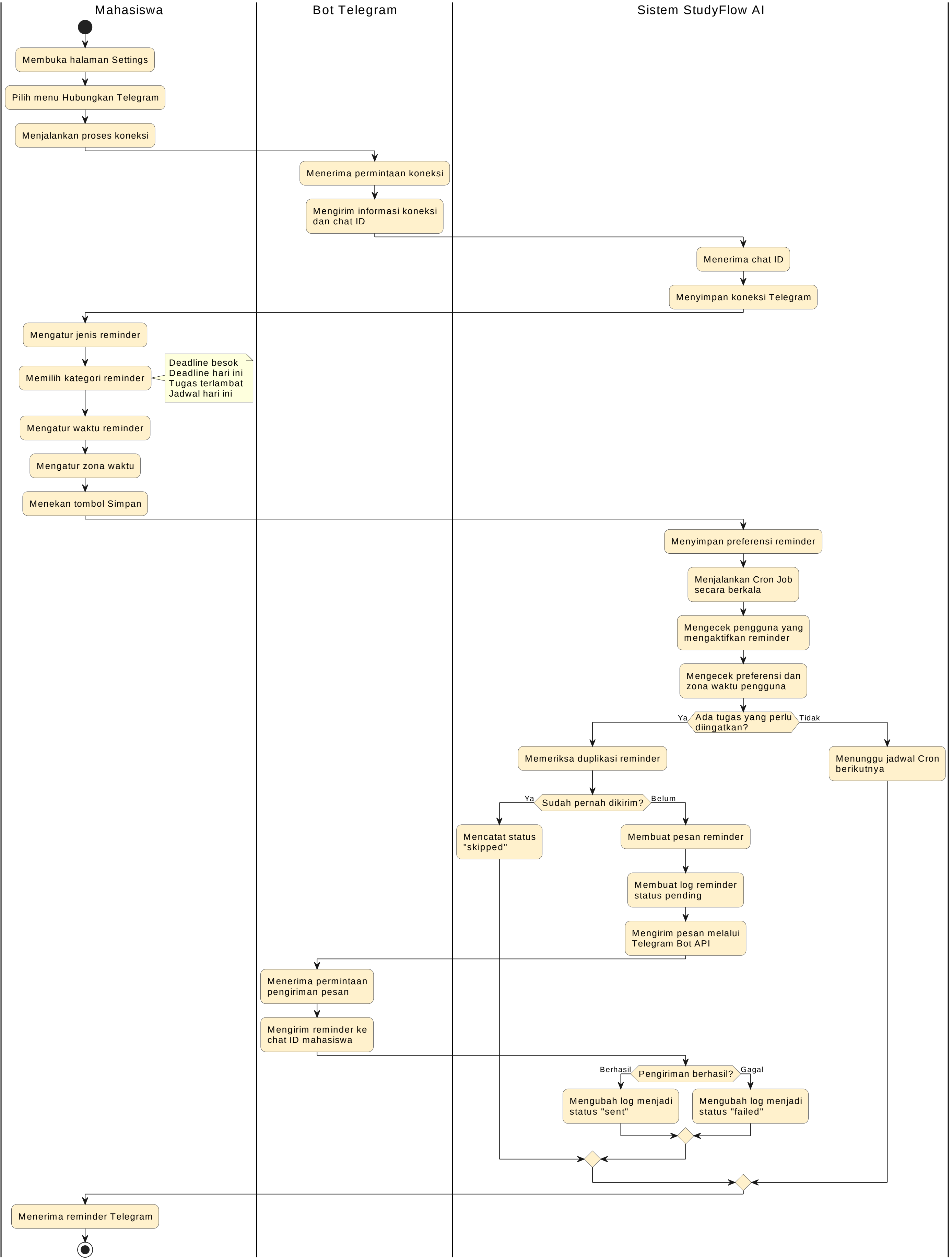
Activity Diagram - Mengatur Reminder Telegram
